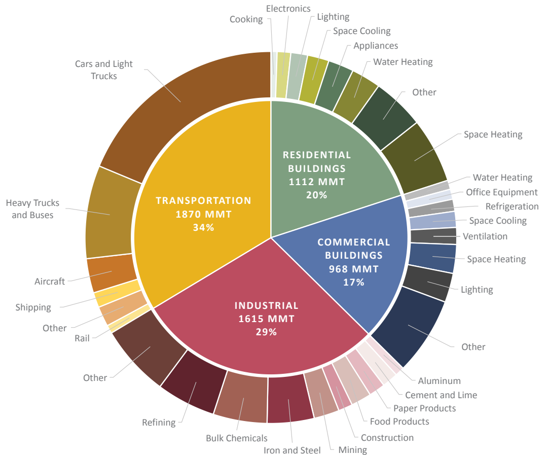
FIGURE 4.2: CO 2 EMISSIONS BY SECTOR AND END USE WITH ELECTRICITY EMISSIONS DISTRIBUTED ACROSS END-USE SECTORS, 2014
