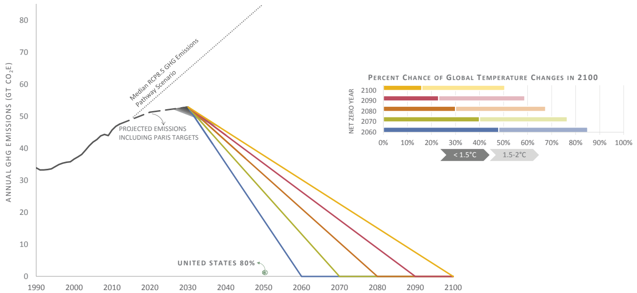
FIGURE E11: GLOBAL TRAJECTORIES TO NET-ZERO GHG EMISSIONS AND PROBABILITY OF GLOBAL TEMPERATURE CHANGES
