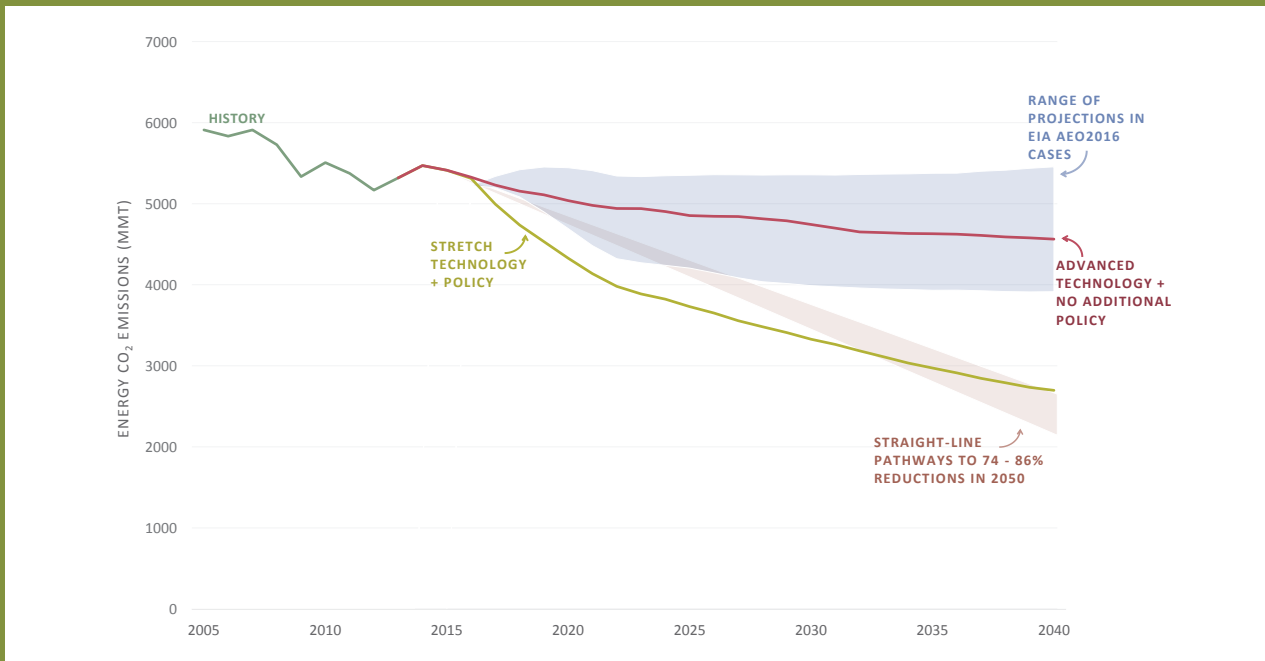
MCS scenarios in GCAM that achieve 80 percent reductions in economy-wide net GHG emissions show energy CO 2 reductions of 74 to 86 percent.
