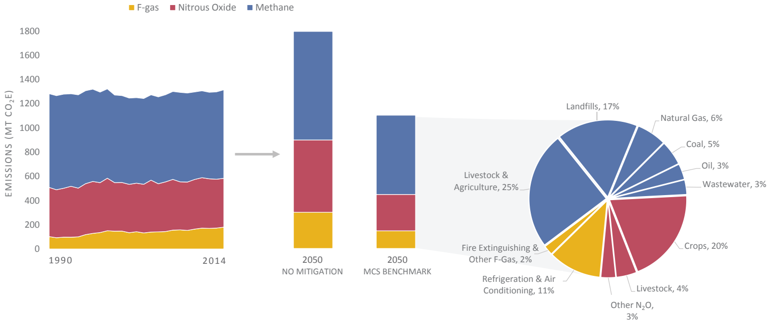
FIGURE 6.2: NON-CO 2 EMISSIONS REDUCTIONS IN 2050 WITH MCS BENCHMARK SCENARIO
