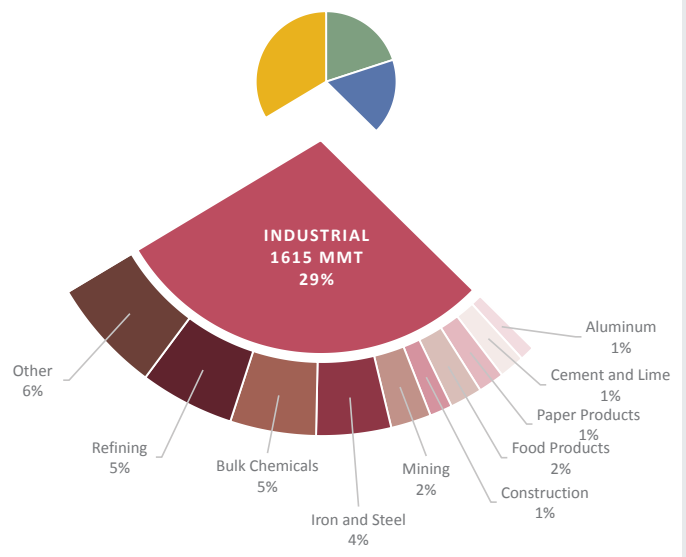
FIGURE 4.16: CO 2 EMISSIONS BY END USE: INDUSTRIAL
