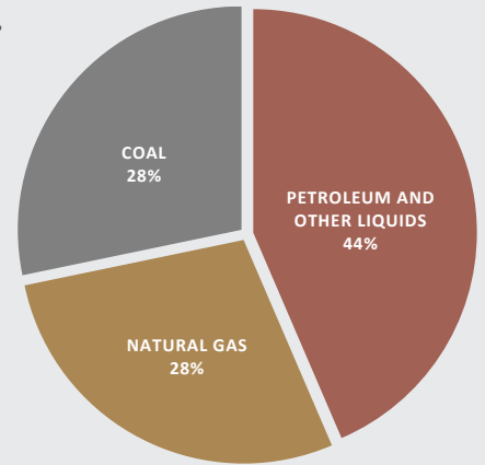
FIGURE 4.1: U.S. CO 2 EMISSIONS FROM ENERGY CONSUMPTION BY FUEL, 2015 (EIA 2016D)
